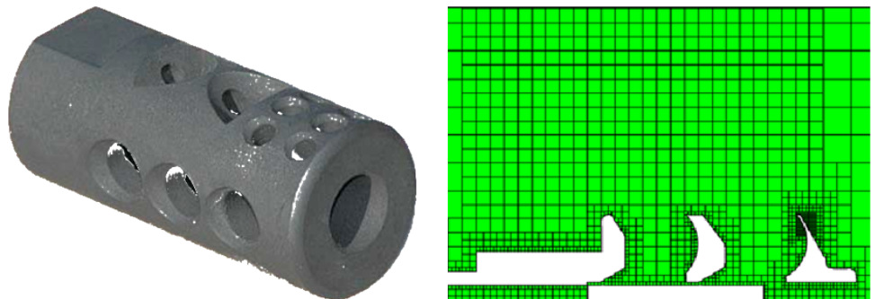
Figure 48: (a) A typical muzzle brake (b) Adaptive grid generated around a muzzle brake
