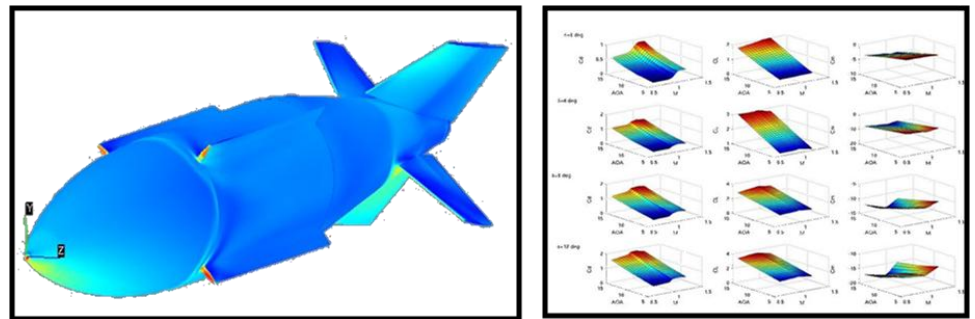
Figure 15: Aerodynamic derivatives of HSLD bomb
